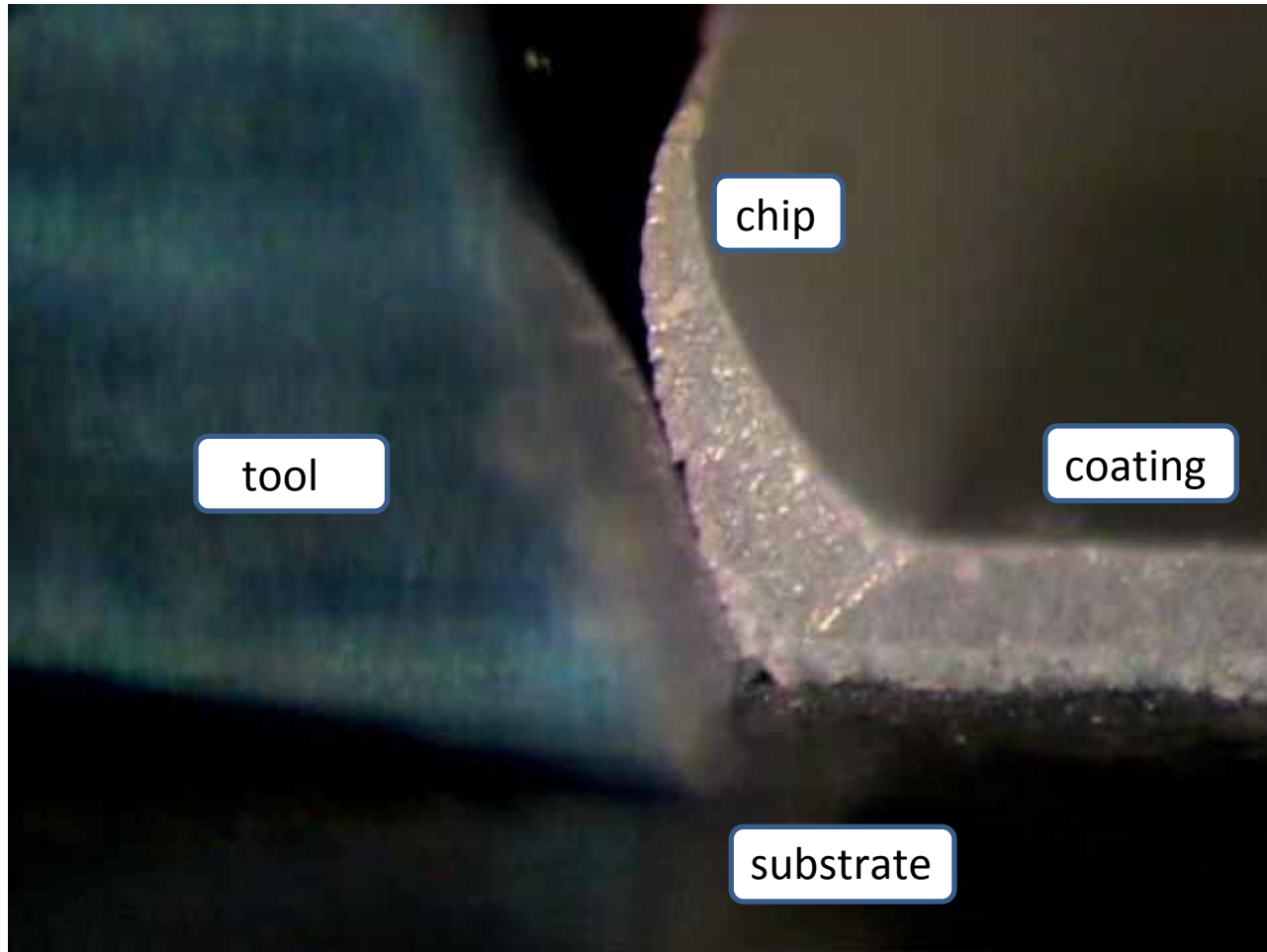
Figure 6 Side view of removing of coating by tool
