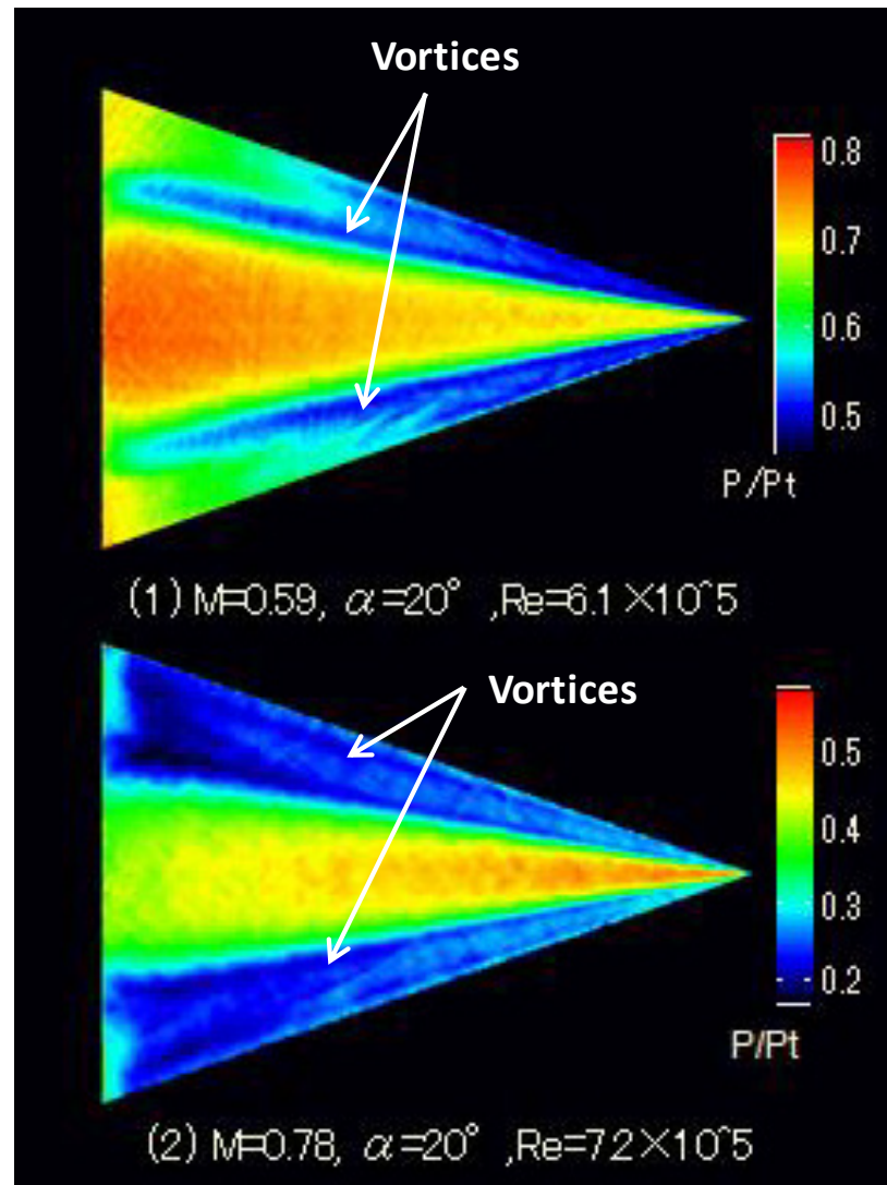
Fig. 10 Pressure distribution on delta wing at (1) M=0.59 and \alpha=20^\circ , Re=6.1 \times 10^5 and (2) M=0.78 , \alpha=20^\circ , Re=7.2 \times 10^5
